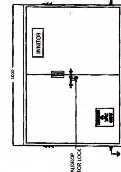
FRONT VIEW WITH DOOR
